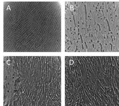
Figure 2. Reconstructed 2D slices of the same sample, captured at the ForMAX beamline, MAX IV Synchrotron. Sample directly frozen (A), annealed at -9 °C (B), partly dried with ice, (C), dried sample (D).
